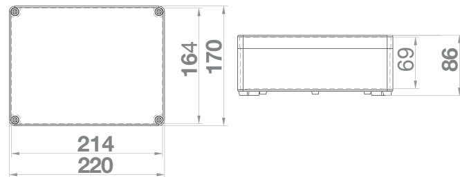
Krabice SolidBOX IP65 - Obj.č. / Item 68161
