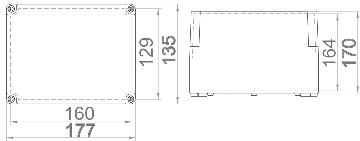
Krabice SolidBOX IP65 - Obj.č. / Item 68151
