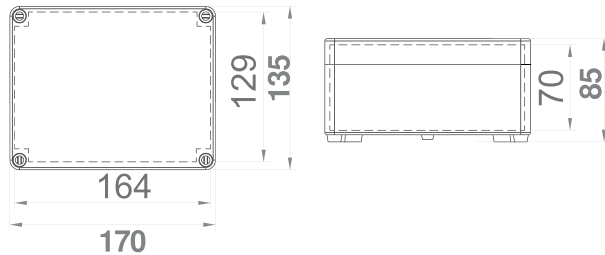
Krabice SolidBOX IP65 - Obj.č. / Item 68121
