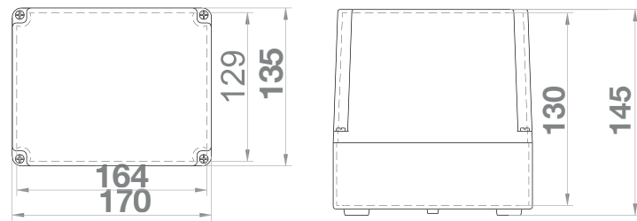
Krabice SolidBOX IP65 - Obj.č. / Item 68140
