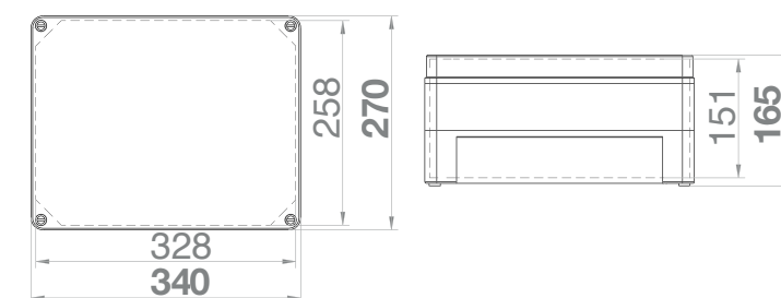
Krabice SolidBOX IP65 - Obj.č. / Item 68271
