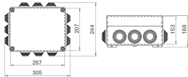
Krabice SolidBOX IP55 - Obj.č. / Item 68232
