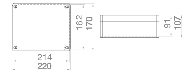
Krabice SolidBOX IP65 - Obj.č. / Item 68171
