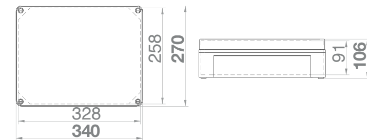
Krabice SolidBOX IP65 - Obj.č. / Item 68251
