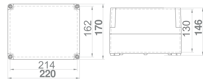
Krabice SolidBOX IP65 - Obj.č. / Item 68181
