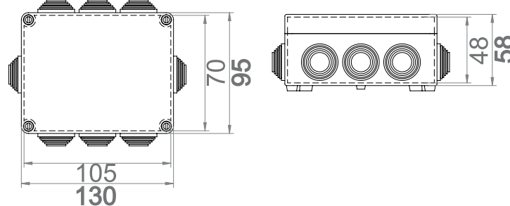
Krabice SolidBOX IP55 - Obj.č. / Item 68052
